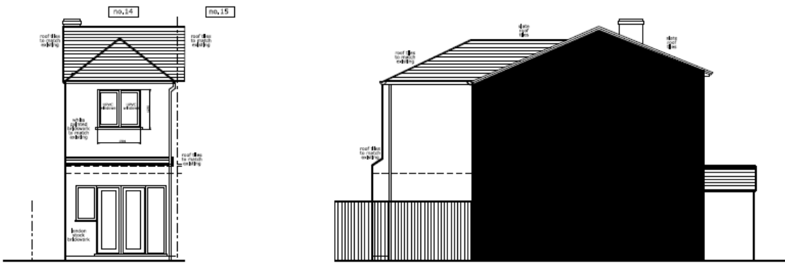
Rear Elevation
