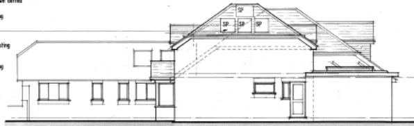
South Elevation
